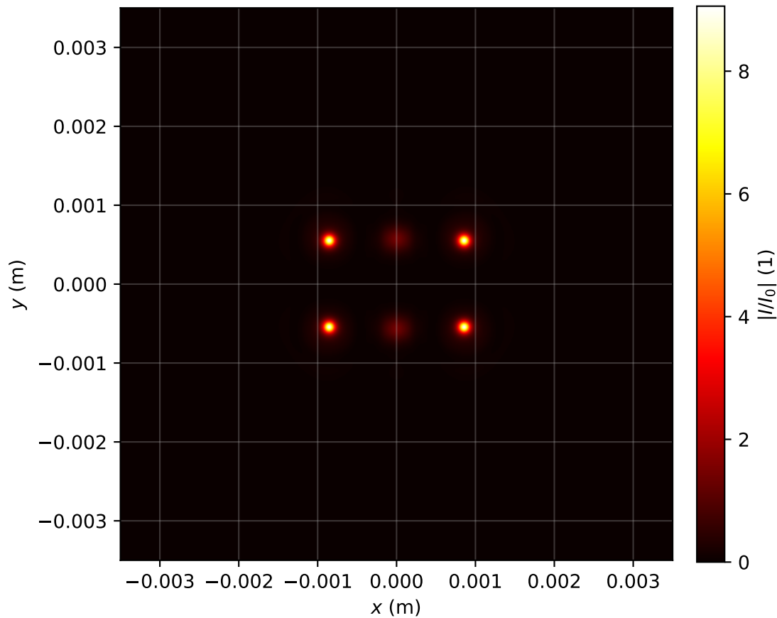
Intensity profile I(x, y, z = 0.796)/I_0 , P_{in}=7.0P_{cr} , artificial time
